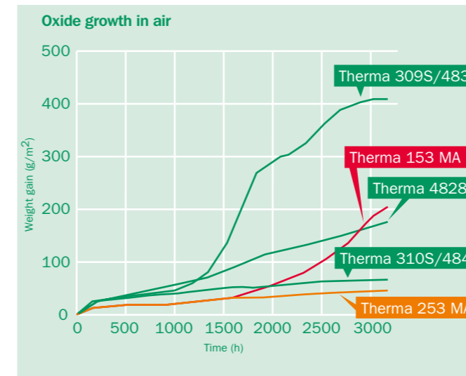
Oxide growth in air at 1000 °C/1830 °F, 165 hour cycles for austenitic high temperature steels.
